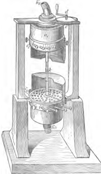
FIG. 124.—Double Syren of von Helmholtz. a_0, a_1 , Brass wind-chests communicating by tubes g_0, g_1 , with bellows; the opposite ends of the cylinders are closed by brass plates perforated with holes corresponding to those seen in the disk, c_0 ; the disks, c_0, c_1 , rotate on a common axis, k , provided with a screw for the counting apparatus, which is omitted here. The upper cylinder, a_1 , can be rotated on a vertical axis in either direction by toothed wheel, e , with handle, d ; the four rows of holes may be opened or shut by means of studs, i, i ; there are 8, 10, 12, and 18 holes respectively in the four rows of holes in the lower disk, and 9, 12, 15, and 16 in the upper (not seen in diagram).
